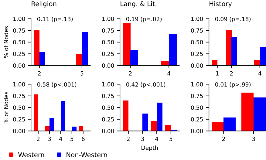
Figure 4.6: Level bias statistics for the topics religion, language & literature, and history in the LCC (top) and the DDC (bottom). Each plot is annotated with the JSD between the Western and non-Western distributions and the significance of the JSD in brackets. Significance was calculated with a permutation test.
