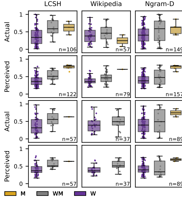
Figure 3.2: Distribution of actual and perceived gender base rates of various jobs across cases W , WM , and M in the LCSH, Wikipedia, and Ngram-D. The top two rows include categories for which we have actual (top row) or perceived (second row) base rates. The bottom rows include categories for which we have both actual and perceived base rates.
