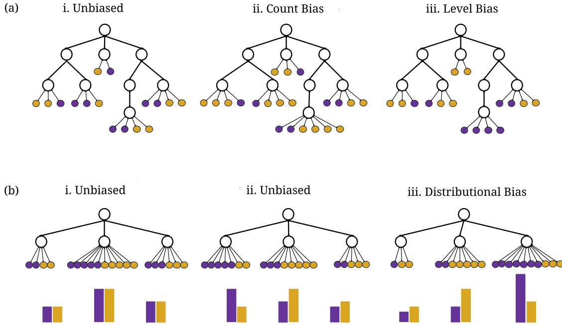
Figure 4.3: An illustration of (a) item count bias and level bias, and (b) distributional bias. In (a), there is (i) a classification with no level or count bias; (ii) a classification with count bias; and (iii) a classification with level bias. In (b), there are (i, ii) two examples of categorizations without distributional bias, and (iii) an example of distributional bias. The shapes of the distributions of purple and gold items across the three lowest categories in the tree are shown with bar graphs. All 3 item biases demonstrate bias against purple items and in favour of gold items.
