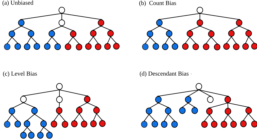
Figure 4.2: An illustration of (a) an unbiased classification, (b) a classification with count bias, (c) a classification with level bias, and (d) a classification with descendant bias. The three category biases demonstrate bias against blue categories and in favour of red categories. White categories cannot be categorized as either red or blue.
