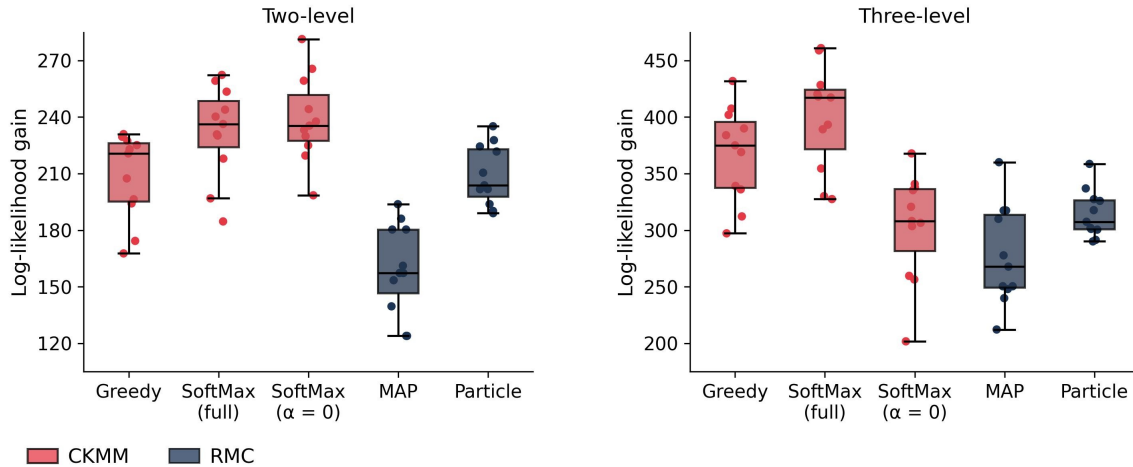
Figure 5.10: Log-likelihood gain over random baseline for CKMM and RMC models on held-out folds ( n = 15 per fold). Results are reported separately for the two-level and three-level conditions. Log-likelihoods are reported as gain over the log-likelihood of the data under random assignment to categories ( -428.5 for two-level systems and -758.9 for three-level systems). Results are from an 11-fold cross-validation.
